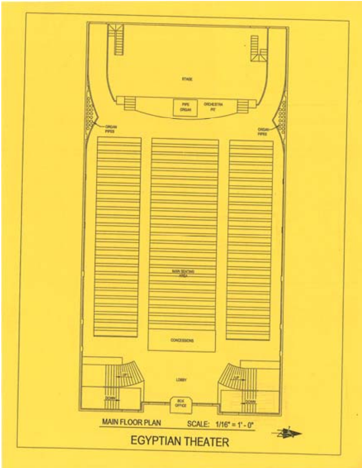
3. Main Floor Plan, Egyptian Theatre
