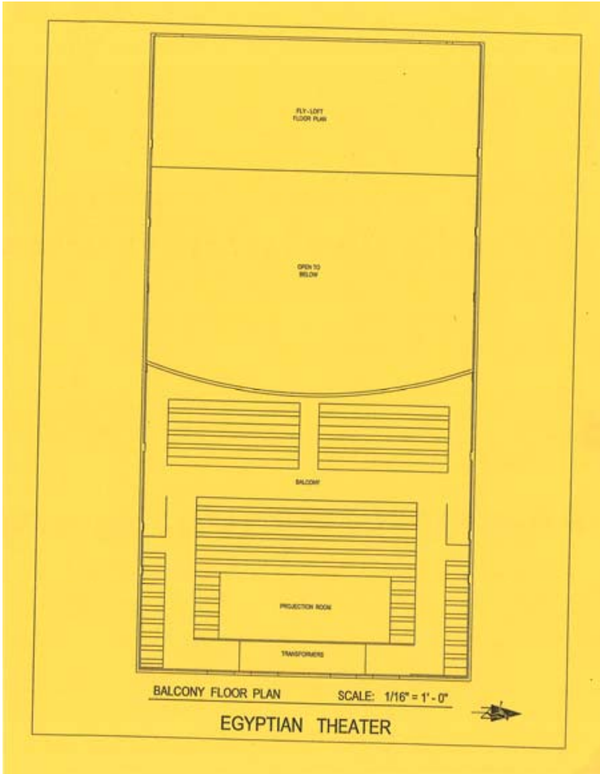
5. Balcony Floor Plan, Egyptian Theatre
